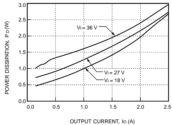
Figure 51. LC010F Typical Power Dissipation vs. Output Current at T_c = 25\text{ }^\circ\text{C}
