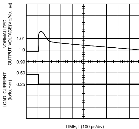
Figure 30. Single-Output Typical Output Voltage for Step Load Change from 50% to 25% of I_o = I_{o, max}
