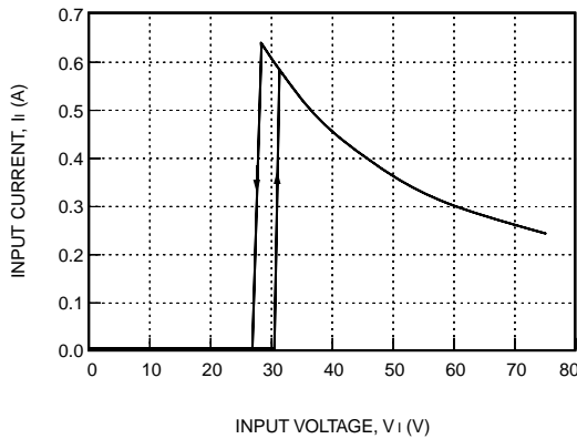
Figure 4. LW015 Input Current vs. Input Voltage at I_{o1} = I_{o, max} and T_c = 25^\circ C
