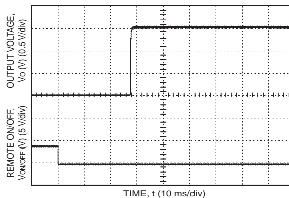
Figure 12. Start-up from Remote On/Off ( I_O = I_{O, \text{max}} ).
