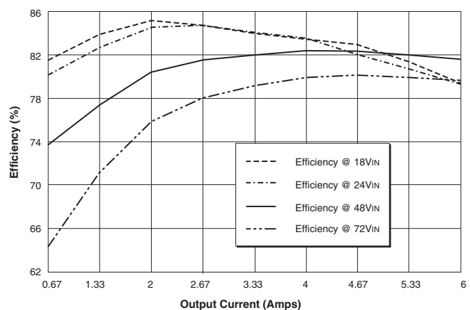
Figure 3c. Efficiency vs. Output Current and Input Voltage
