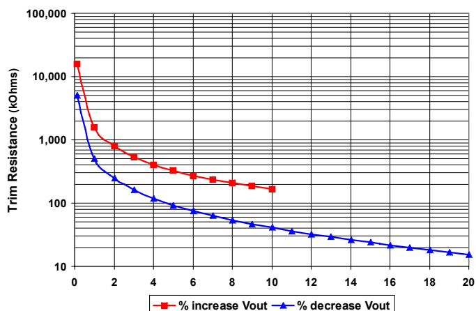
Figure C: Trim Graph for 5.0Vout module
