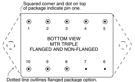
FIGURE 5: PIN OUT TRIPLE OUTPUT MODELS
